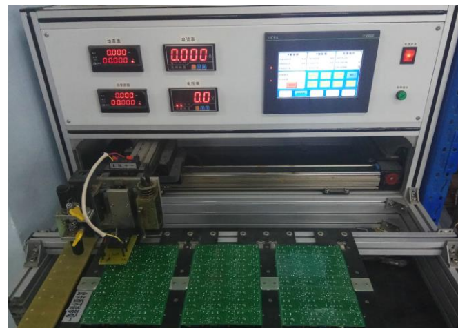
Aging Lines
